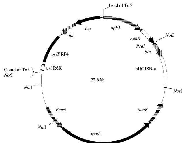
FIG. 1. pLANT3 plasmid restriction map. PstI , salicylate-induced promoter; Penst , constitutive promoter of B. cepacia PR1 23 (TOM 23C ); tomA , Tom gene; tomB , catechol 2,3-dioxygenase gene; trp , transposase gene; bla , \beta -lactamase gene which confers ampicillin resistance; aphA , aminoglycoside 3'-phosphotransferase A gene from Tn903 which confers kanamycin resistance; ori R6K , R6K origin of replication; oriT RP4 , mobilizing region. The region between the I and O ends of Tn5 is transposed.
